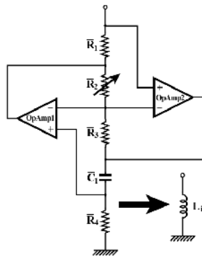
Fig. 5. Synthetic inductor.
